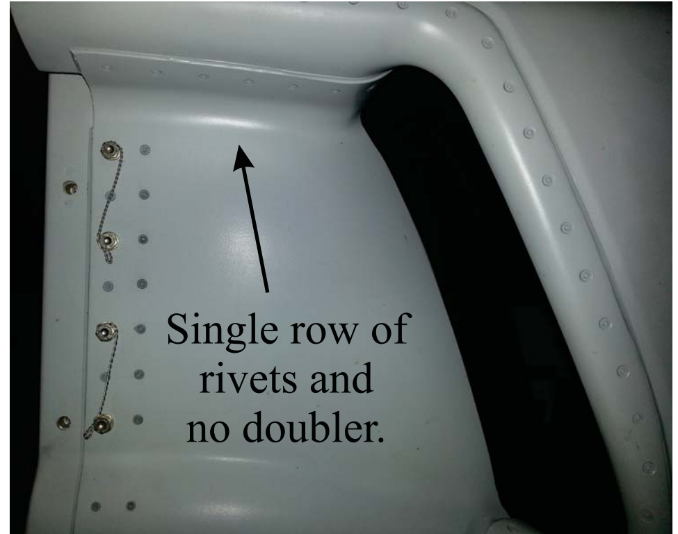
Carbon Fiber (New Style) Bell P/N 407-064-004-101
