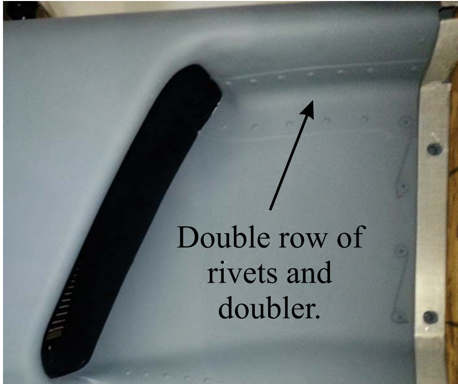
Aluminum (Old Style)
